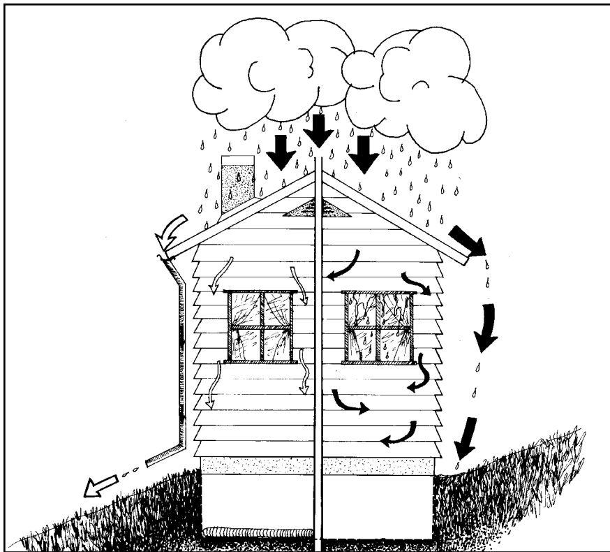
Figure 10 Gutters, a slope away from the house, and drainage tile in the foundation keep the left side of this house dry. No gutters, a slope toward the house, and no drainage tile expose the right side to moisture damage.
