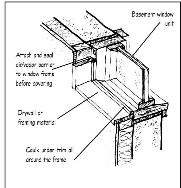
Figure 9 Seal around window and door openings.
