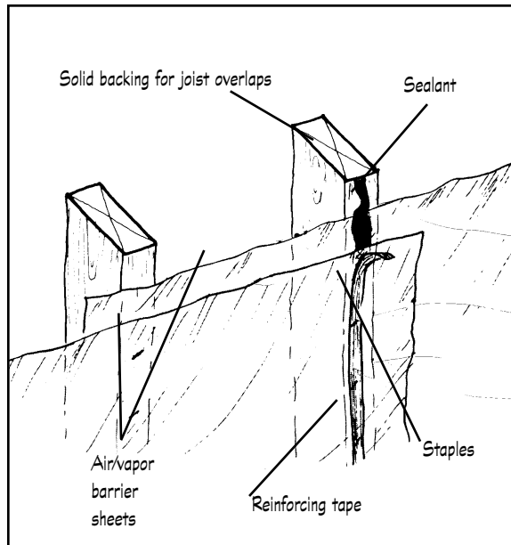
Figure 8 Overlap the air/vapor barrier at least one joist or stud space. (Insulation is not shown.)
